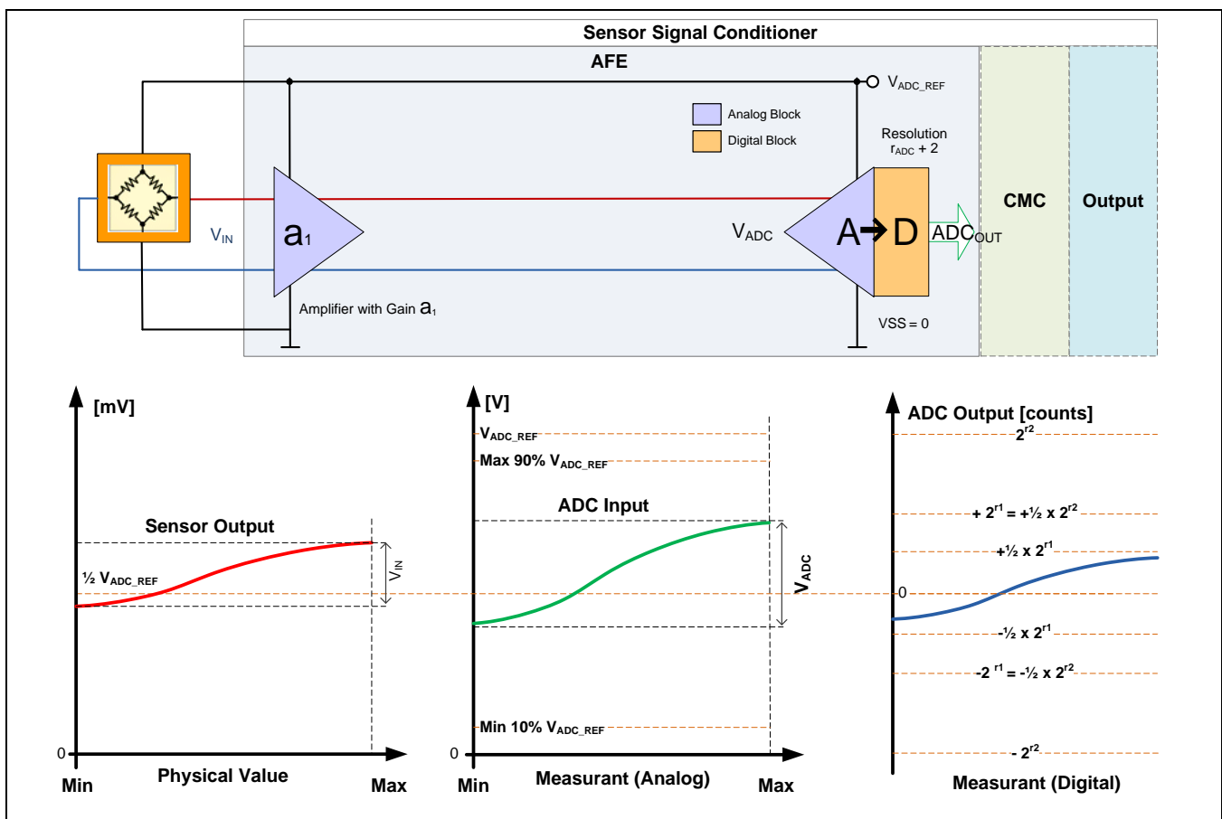
Figure 2.2 Range Zooming
