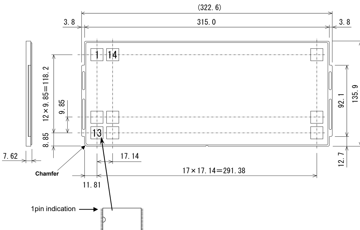
Figure : Dimension of tray and the method to pack ICs (Unit : mm)
