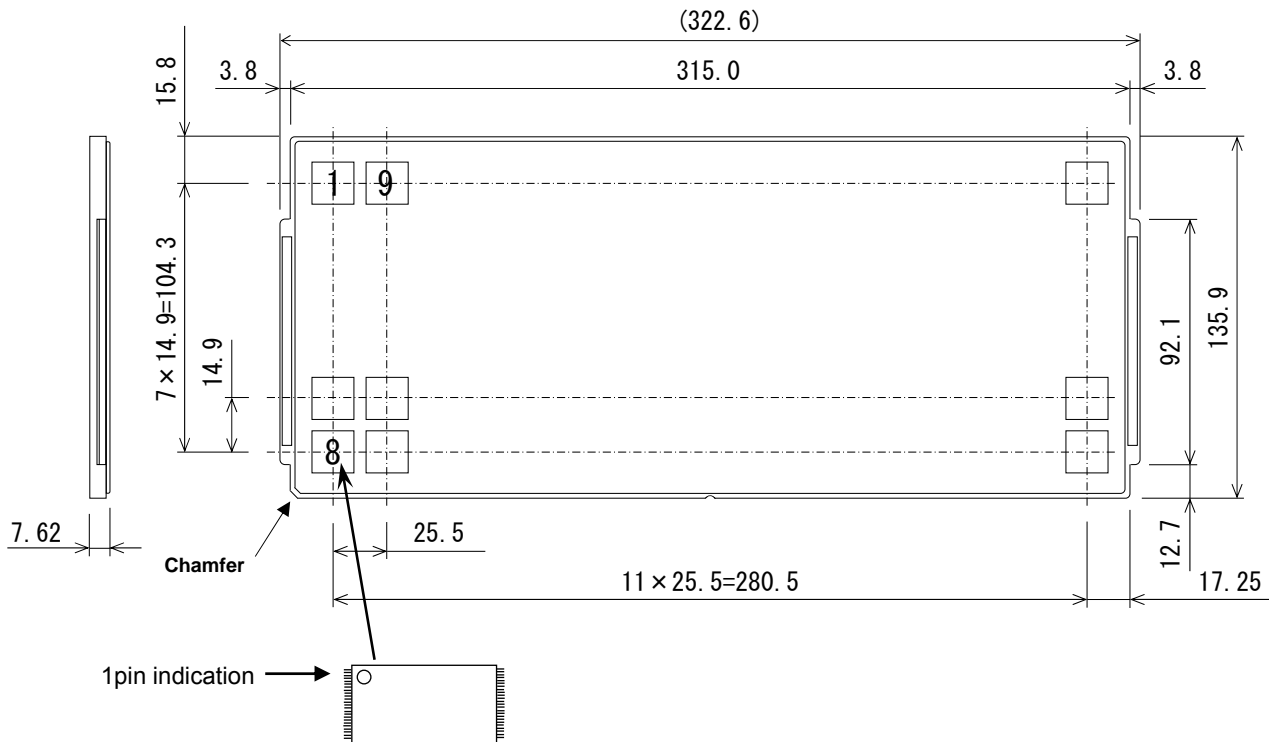
Figure : Dimension of tray and the method to pack ICs (Unit : mm)
