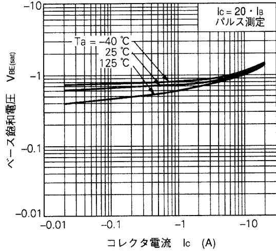
BASE SATURATON VOLTAGE vs. COLLECTOR CURRENT
