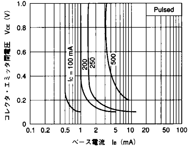
COLLECTOR TO EMITTER VOLTAGE vs. BASE CURRENT
