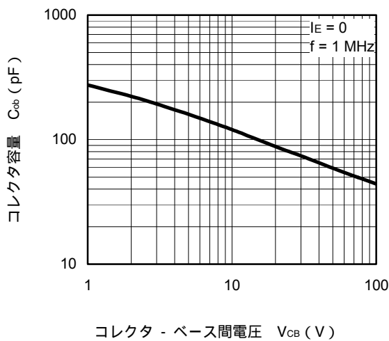
COLLECTOR CAPACITANCE vs. COLLECTOR TO BASE VOLTAGE
