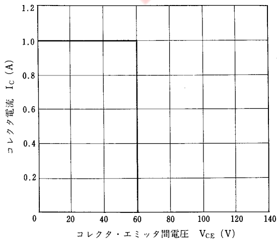
REVERSE BIAS SAFE OPERATING AREAS
