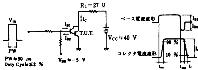
SWITCHING TIME ( t_{on} , t_{stg} , t_f ) TEST CIRCUIT
