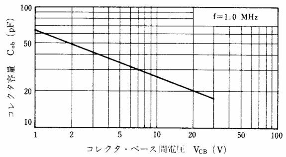
OUTPUT CAPACITANCE vs. COLLECTOR TO BASE VOLTAGE
