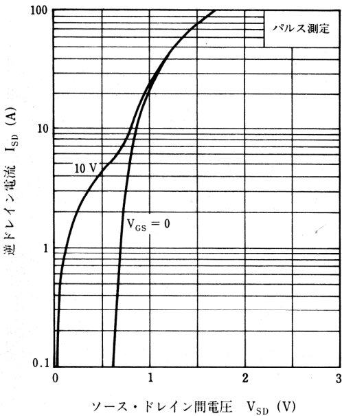
SOURCE TO DRAIN DIODE FORWARD VOLTAGE
