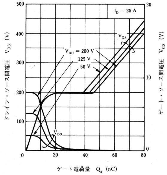
DYNAMIC INPUT CHARACTERISTICS
