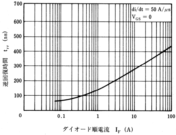
REVERSE RECOVERY TIME vs. REVERSE DRAIN CURRENT
