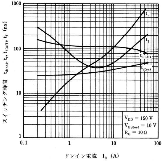
SWITCHING CHARACTERISTICS
