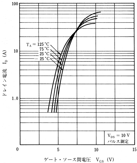
TRANSFER CHARACTERISTICS
