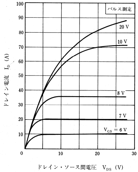
DRAIN CURRENT vs. DRAIN TO SOURCE VOLTAGE
