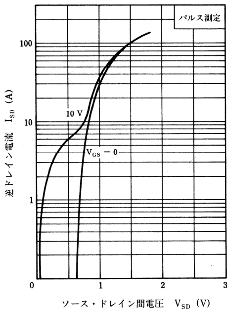
SOURCE TO DRAIN DIODE FORWARD VOLTAGE
