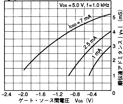
FORWARD TRANSFER ADMITTANCE ( y_{fs} ) vs. GATE TO SOURCE VOLTAGE
