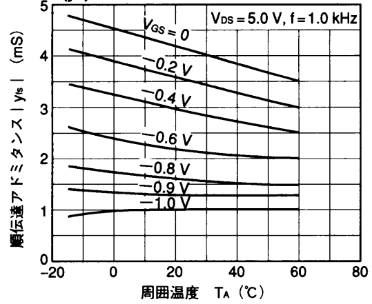
FORWARD TRANSFER ADMITTANCE ( y_{fs} ) vs. AMBIENT TEMPERATURE
