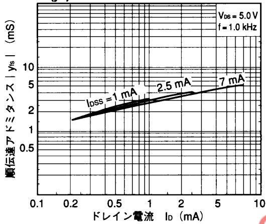
FORWARD TRANSFER ADMITTANCE ( y_{fs} ) vs. DRAIN CURRENT
