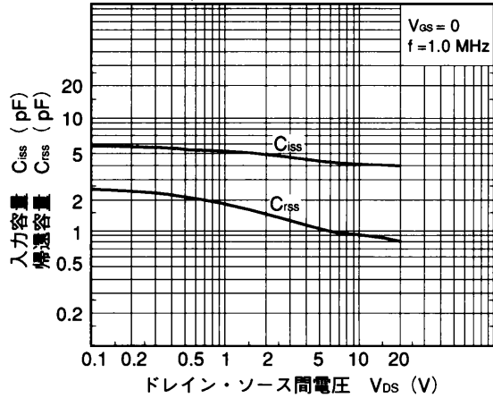
INPUT AND REVERSE TRANSFER CAPACITANCE vs. DRAIN TO SOURCE VOLTAGE
