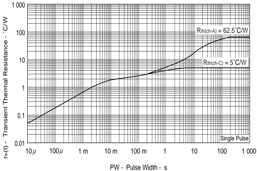
TRANSIENT THERMAL RESISTANCE vs. PULSE WIDTH
