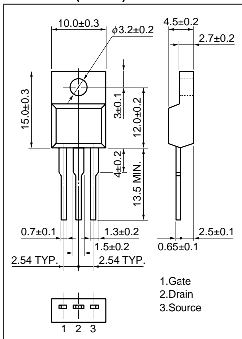
Isolated TO-220 (MP-45F)
