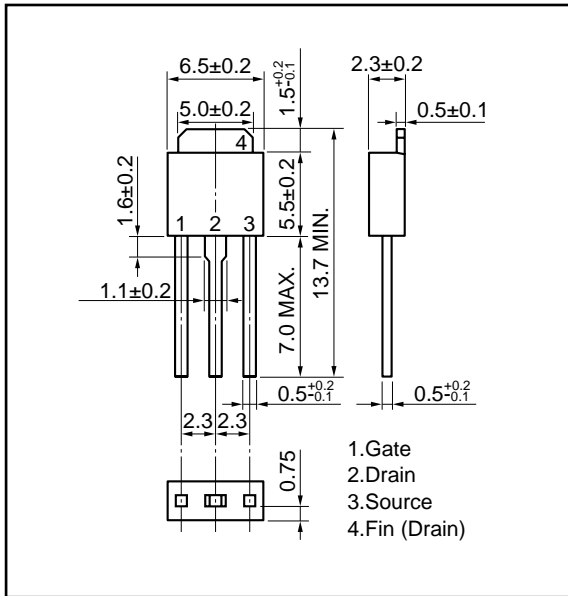
1)TO-251 (MP-3)
