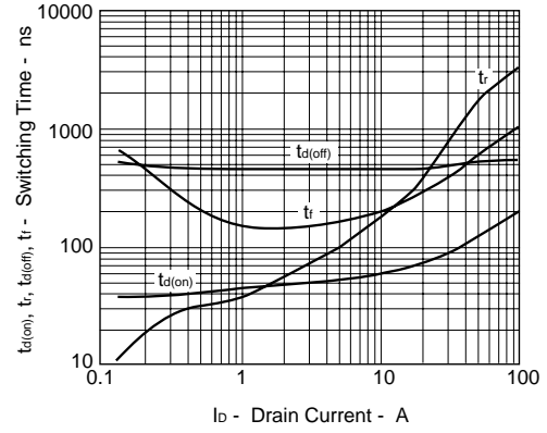
SWITCHING CHARACTERISTICS
