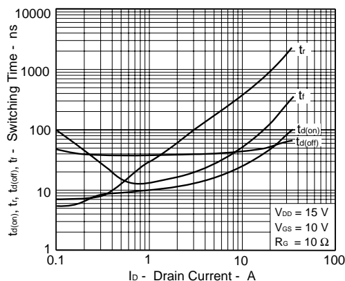
SWITCHING CHARACTERISTICS
