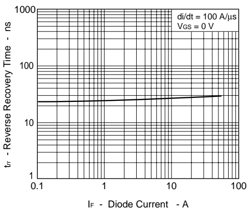
REVERSE RECOVERY TIME vs. DIODE CURRENT
