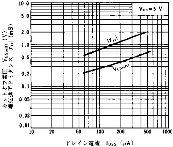
FORWARD TRANSFER ADMITTANCE AND GATE TO SOURCE CUTOFF VOLTAGE vs. ZERO-GATE VOLTAGE DRAIN CURRENT
