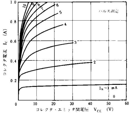
2SC2690, 2SC2690A COLLECTOR CURRENT vs. COLLECTOR TO EMITTER VOLTAGE
