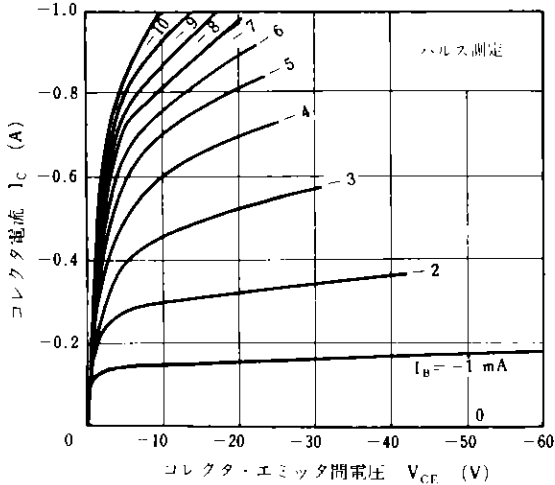
2SA1220, 2SA1220A COLLECTOR CURRENT vs. COLLECTOR TO EMITTER VOLTAGE
