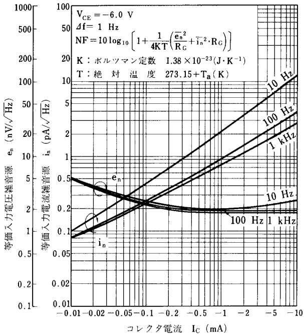
EQUIVALENT INPUT VOLTAGE NOISE SOURCE vs. COLLECTOR EQUIVALENT INPUT CURRENT NOISE SOURCE vs. CURRENT
