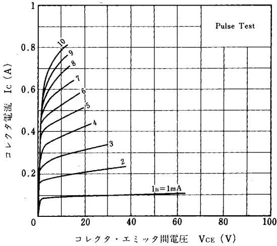
2SD414, 2SD415 COLLECTOR CURRENT vs. COLLECTOR TO EMITTER VOLTAGE
