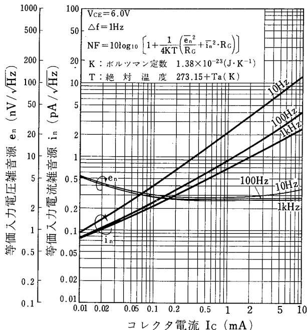
EQUIVALENT INPUT VOLTAGE NOISE SOURCE vs. COLLECTOR CURRENT EQUIVALENT INPUT CURRENT NOISE SOURCE vs. COLLECTOR CURRENT
