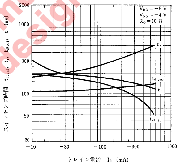
SWITCHING CHARACTERISTICS
