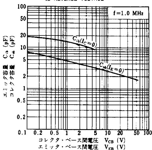
INPUT AND OUTPUT CAPACITANCE vs. REVERSE VOLTAGE
