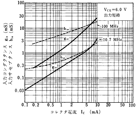
INPUT ADMITTANCE ( y_{ie} ) vs. COLLECTOR CURRENT
