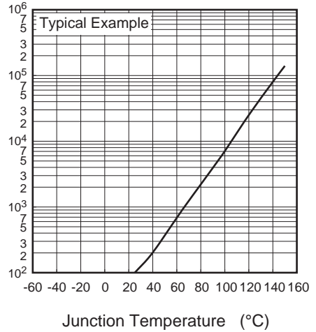
Repetitive Peak Off-State Current vs. Junction Temperature
