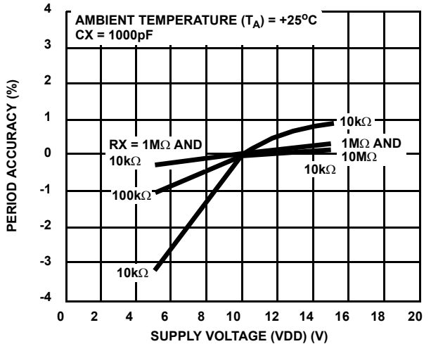
FIGURE 13. TYP. ASTABLE OSCILLATOR OR Q, Q̄ PERIOD ACCURACY vs SUPPLY VOLTAGE
