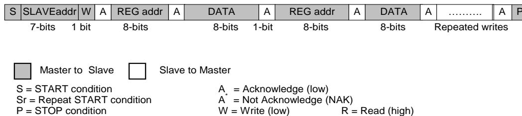
Figure 38: I 2 C Repeated Write (SDA line)
