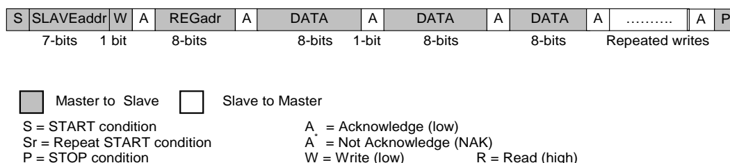
Figure 37: I 2 C Page Write (SDA line)
