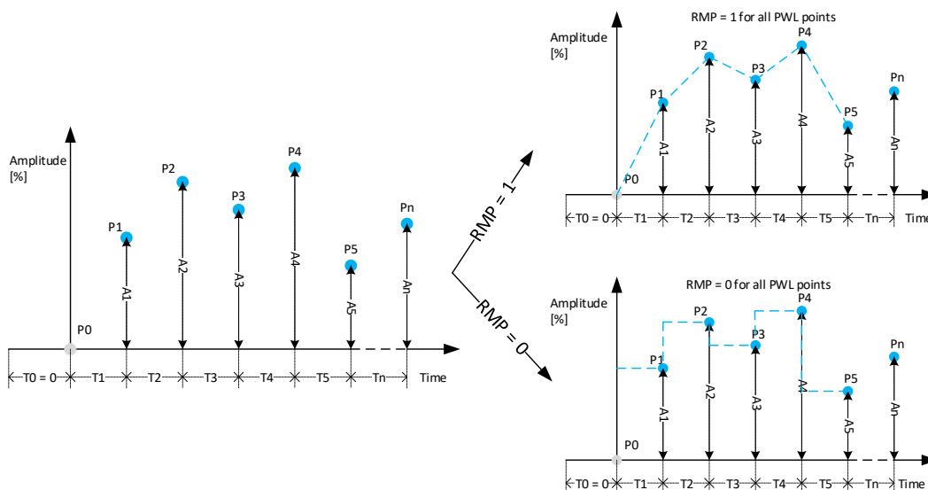
Figure 26: Snippet Example
