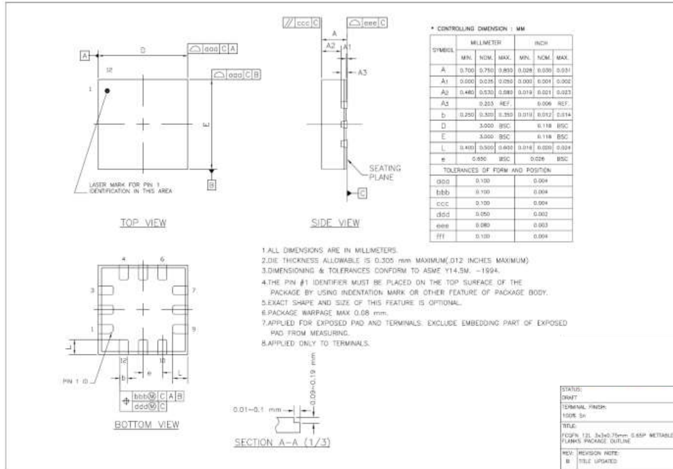
Figure 40: QFN Package Outline Drawing
