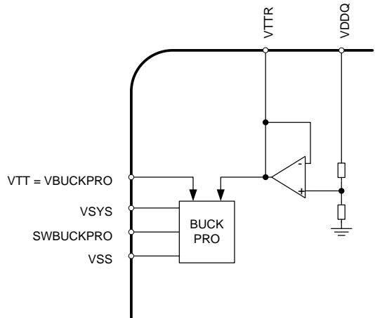
Figure 33: BUCKPRO Memory Bus Termination Mode
