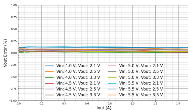
Figure 13. CH1 Buck Load Regulation in PWM Mode
