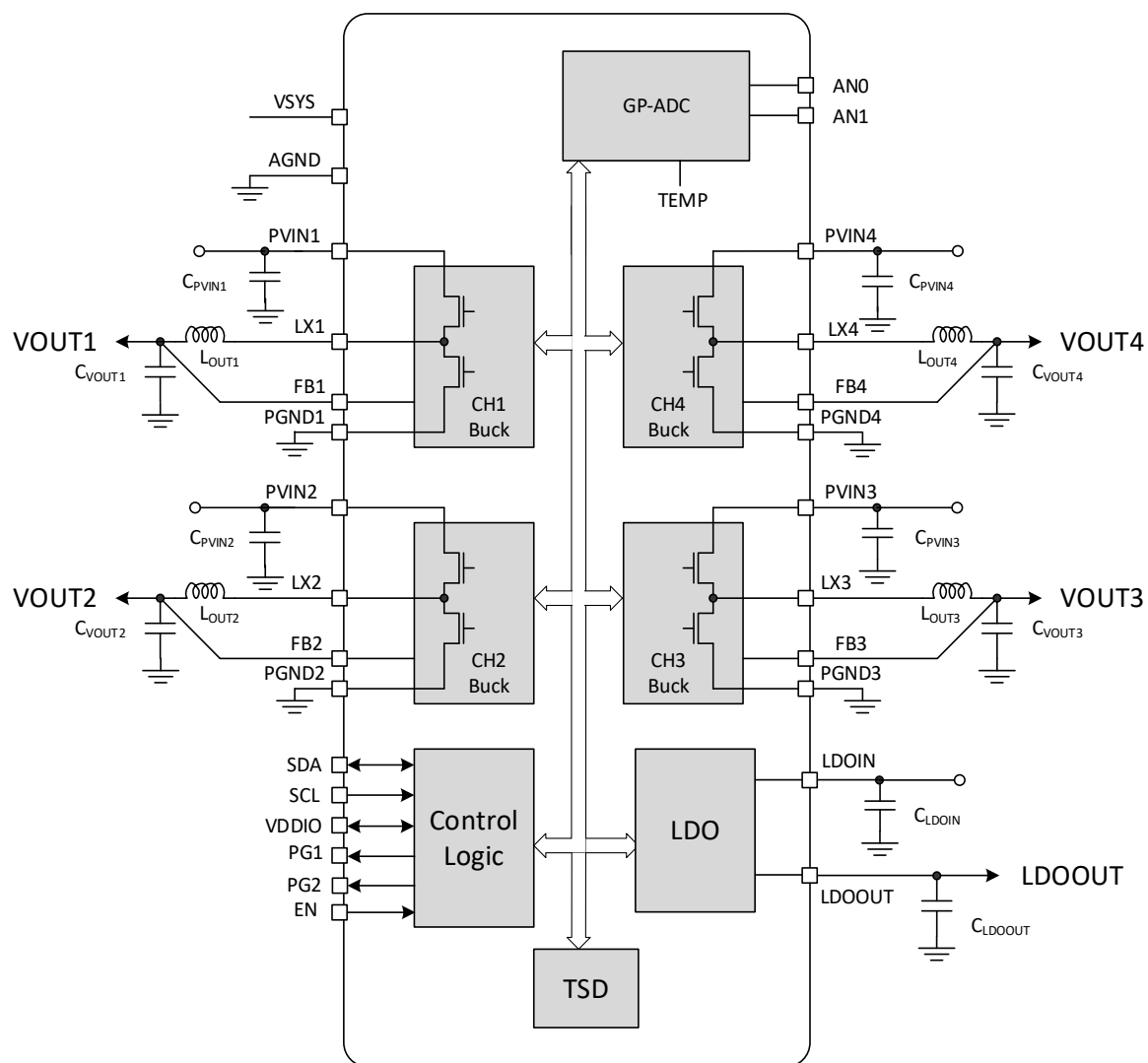
Figure 1. System Diagram
