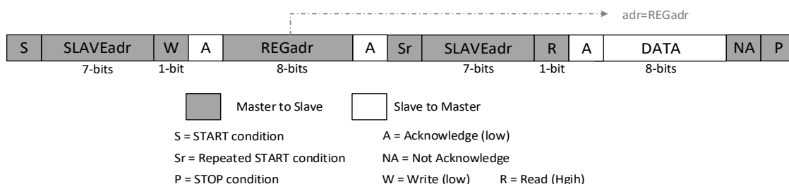
Figure 48. Single Read Command
