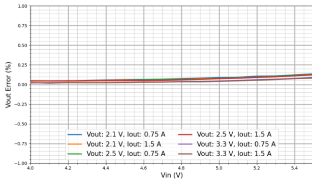
Figure 20. CH1 Buck Line Regulation in Auto Mode
