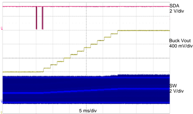
Figure 32: Buck V OUT 1.3 V to 1.9 V; Buck V IN = 3.6 V, Buck I LOAD = 60 mA
