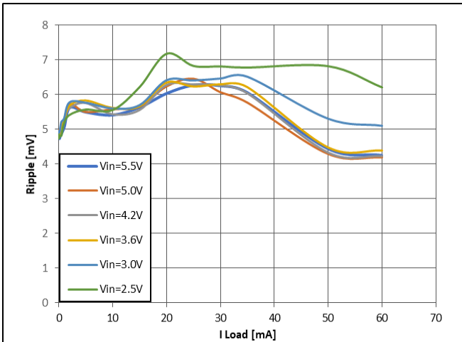
Figure 18: Buck V OUT = 0.9 V
