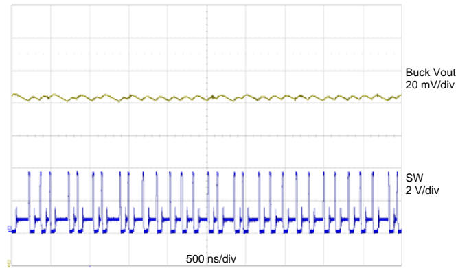
Figure 27: Buck V_{IN} = 3.6\text{ V} , Buck V_{OUT} = 0.7\text{ V} , Buck I_{LOAD} = 60\text{ mA}
