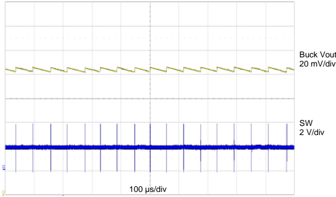
Figure 24: Buck V_{IN} = 3.6\text{ V} , Buck V_{OUT} = 1.8\text{ V} , Buck I_{LOAD} = 1\text{ mA}
