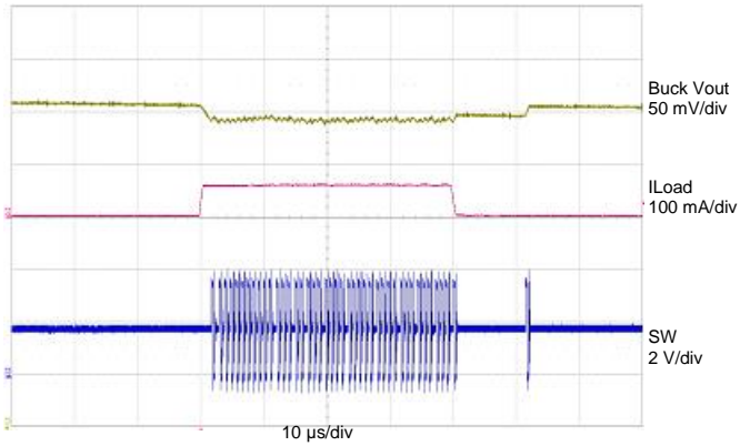
Figure 28: Buck I_{LOAD} = 0.5 \text{ mA} to 60 \text{ mA} to 0.5 \text{ mA} ( 0.1 \text{ A}/\mu\text{s} ); Buck V_{IN} = 3.6 \text{ V} , Buck V_{OUT} = 1.8 \text{ V}
