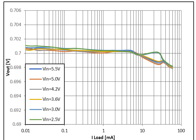
Figure 23: Buck V_{OUT} = 0.7\text{ V}
