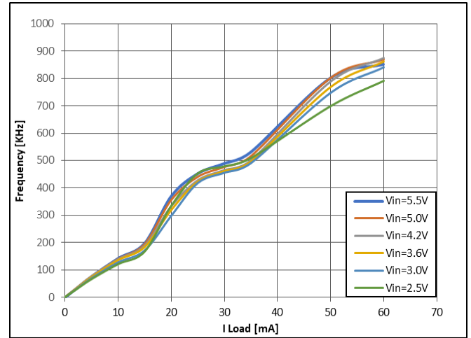
Figure 13: Buck V_{OUT} = 1.2\text{ V}
