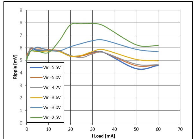
Figure 19: Buck V OUT = 0.7 V
