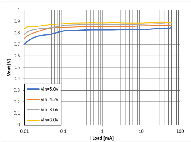
Figure 8: Buck V_{OUT} = 1.8\text{ V}
