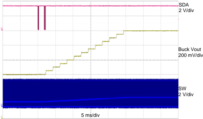
Figure 30: Buck V OUT 0.6 V to 1.2 V; Buck V IN = 3.6 V, Buck I LOAD = 60 mA
