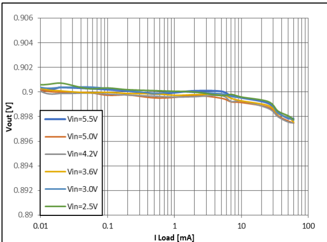
Figure 22: Buck V_{OUT} = 0.9\text{ V}
