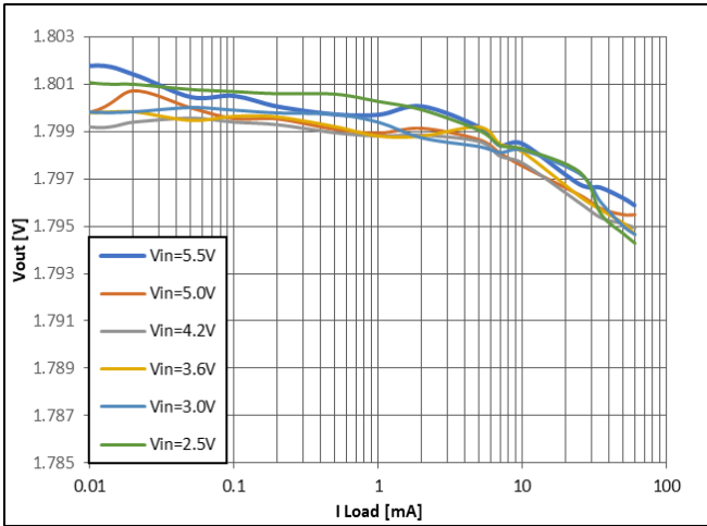
Figure 20: Buck V_{OUT} = 1.8\text{ V}
