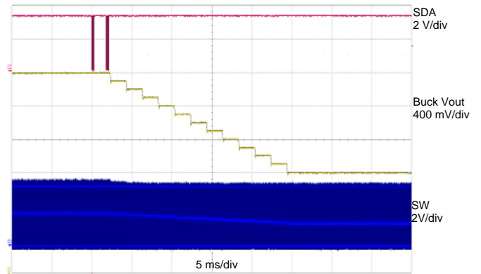
Figure 33: Buck V OUT 1.9 V to 1.3 V; Buck V IN = 3.6 V, Buck I LOAD = 60 mA
