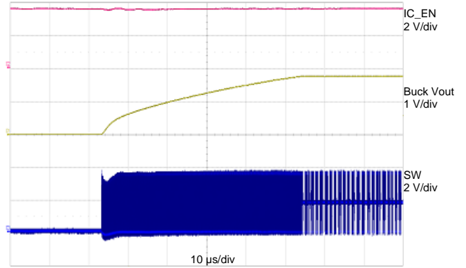
Figure 35: V_{OUT} ramp-up after Enabled (Zoom-in of 34)
