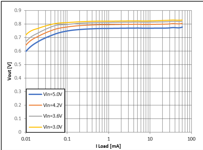
Figure 10: Buck V_{OUT} = 0.9\text{ V}
