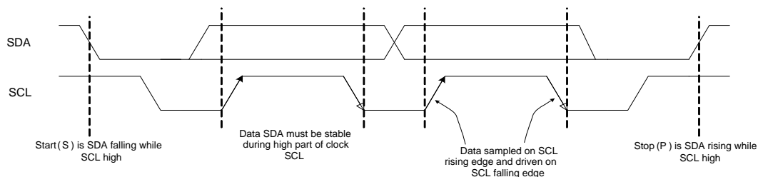
Figure 37: I 2 C Start and Stop Conditions
