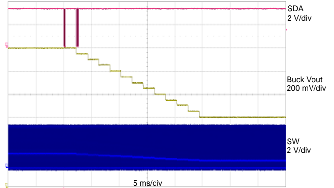
Figure 31: Buck V OUT 1.2 V to 0.6 V; Buck V IN = 3.6 V, Buck I LOAD = 60 mA
