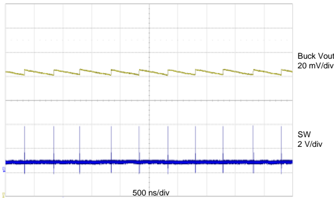
Figure 26: Buck V_{IN} = 3.6\text{ V} , Buck V_{OUT} = 0.7\text{ V} , Buck I_{LOAD} = 1\text{ mA}
