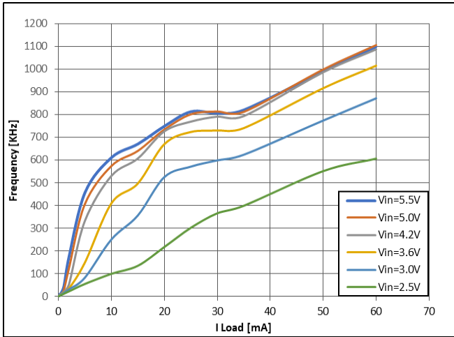
Figure 12: Buck V_{OUT} = 1.8\text{ V}
