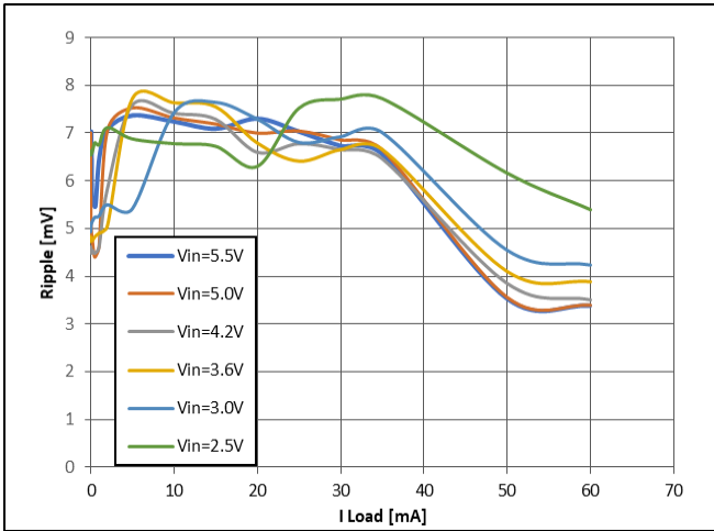
Figure 16: Buck V OUT = 1.8 V
