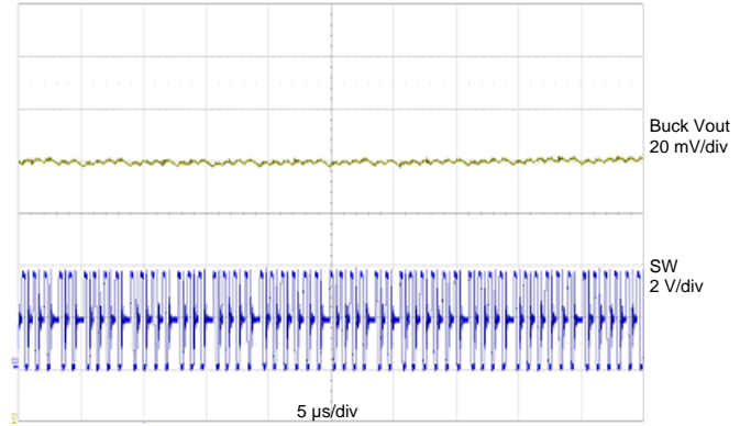
Figure 25: Buck V_{IN} = 3.6\text{ V} , Buck V_{OUT} = 1.8\text{ V} , Buck I_{LOAD} = 60\text{ mA}
