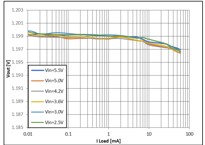
Figure 21: Buck V_{OUT} = 1.2\text{ V}
