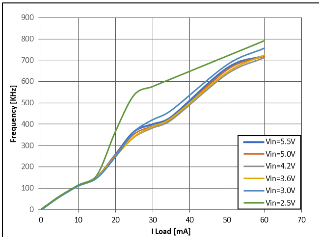
Figure 14: Buck V_{OUT} = 0.9\text{ V}
