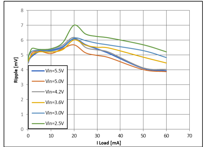
Figure 17: Buck V OUT = 1.2 V
