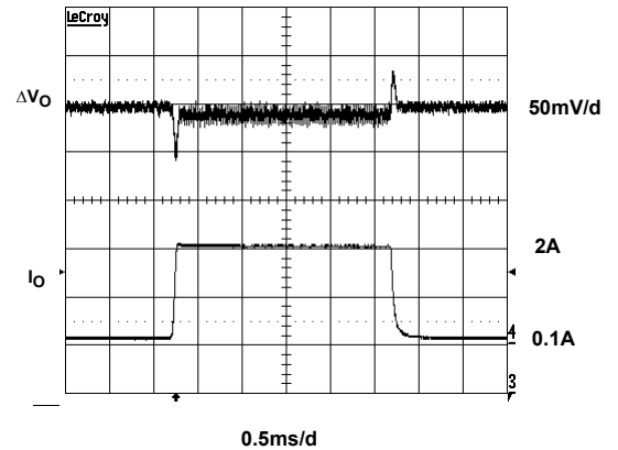
FIGURE 12. TRANSIENT RESPONSE
