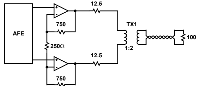
FIGURE 24. CIRCUIT CONFIGURATION
