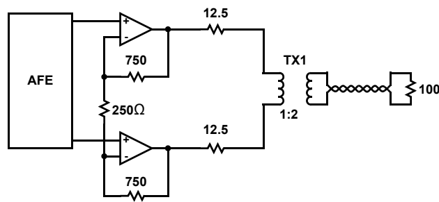
Figure 23. Circuit Configuration
