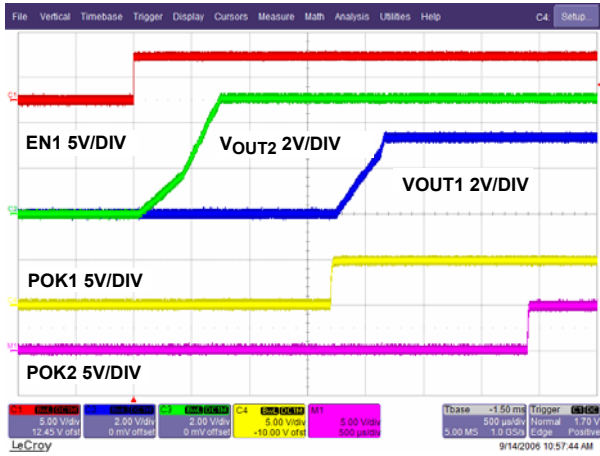
FIGURE 45. DELAYED START-UP ( V_{OUT1} = 5V , V_{OUT2} = 3.3V , EN2 = REF )
