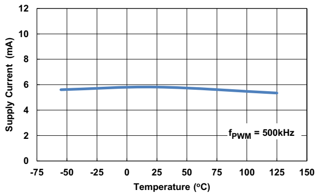
Figure 19. Operating Supply Current vs Temperature
