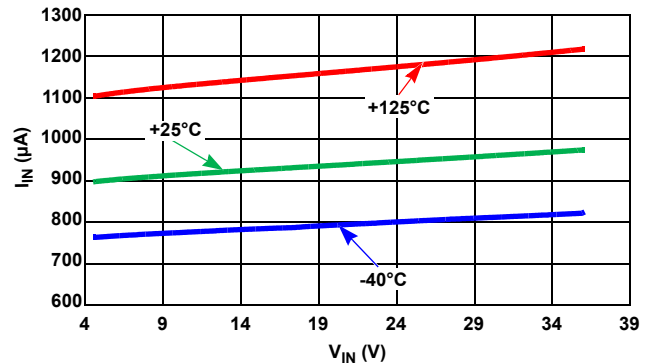
Figure 8. I_{IN} vs V_{IN} , Three Temperatures
