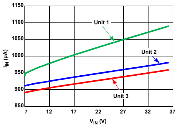
Figure 7. I_{IN} vs V_{IN} , Three Units
