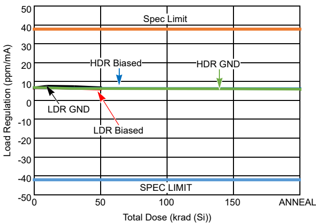
Figure 10. Load Regulation (Sinking) Shift
