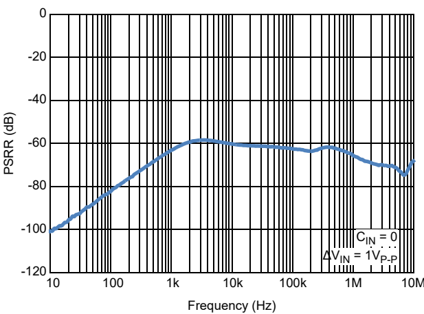
Figure 22. Ripple Rejection vs Frequency
