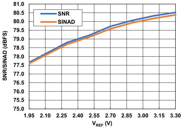
Figure 43. SNR and SINAD vs V REF
