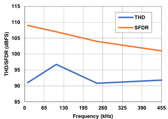
Figure 18. THD and SFDR vs Frequency
