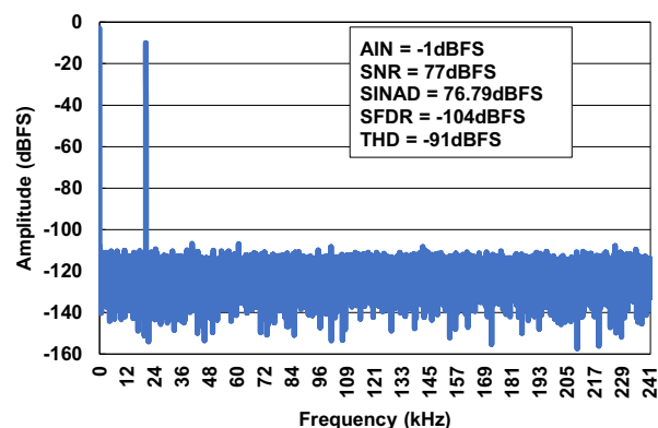
Figure 2. FFT - 20.3kHz
