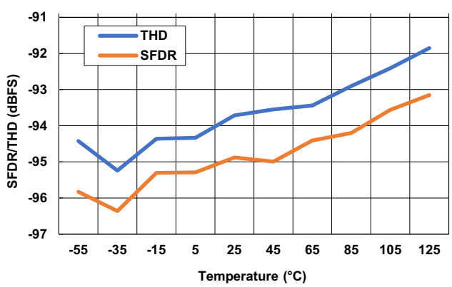
Figure 78. SFDR and THD vs Temperature - PGA Bypassed
