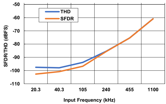
Figure 100. SFDR and THD vs Frequency
