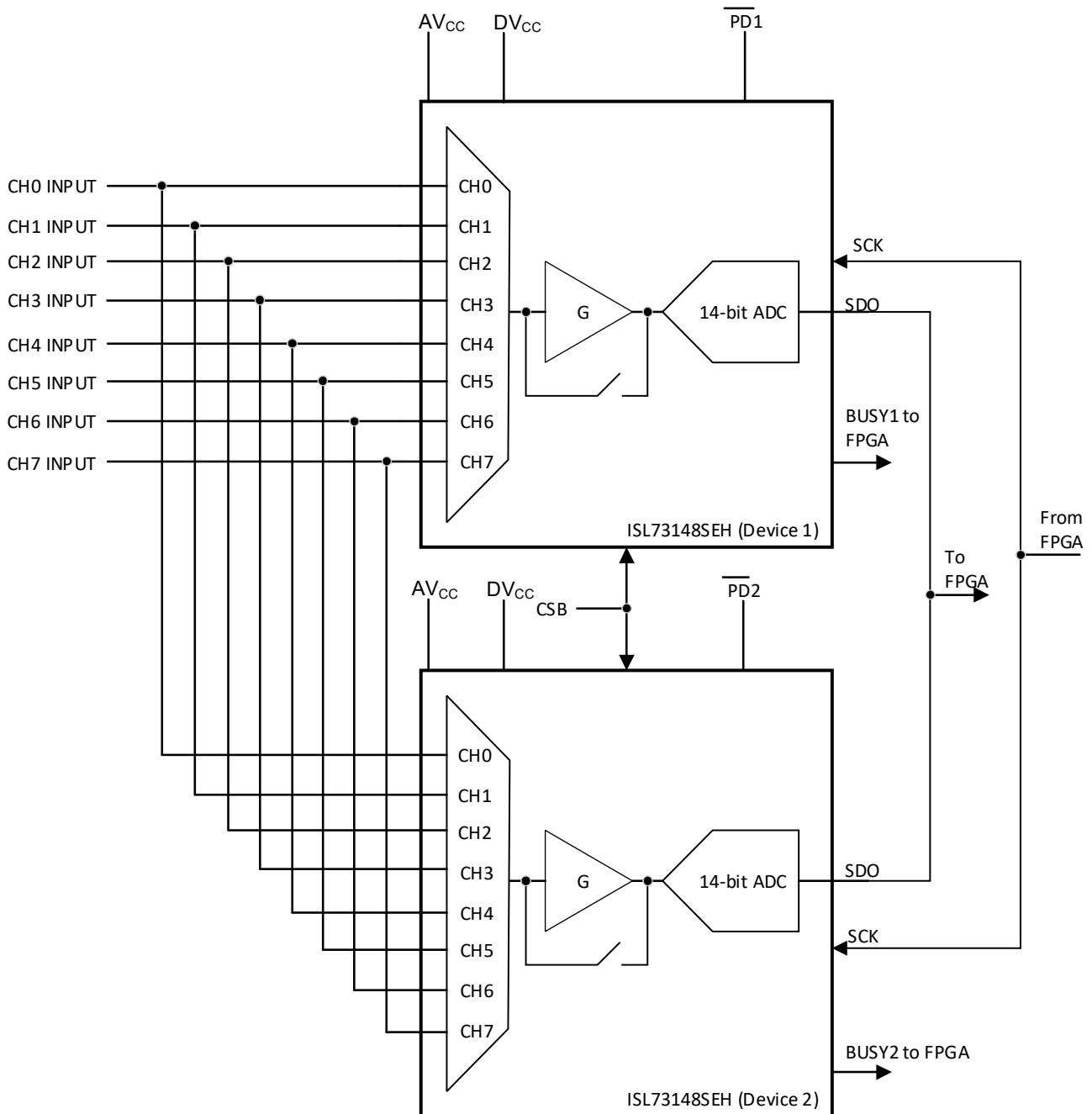
Figure 126. ISL73148SEH Cold Sparring Example Circuit
