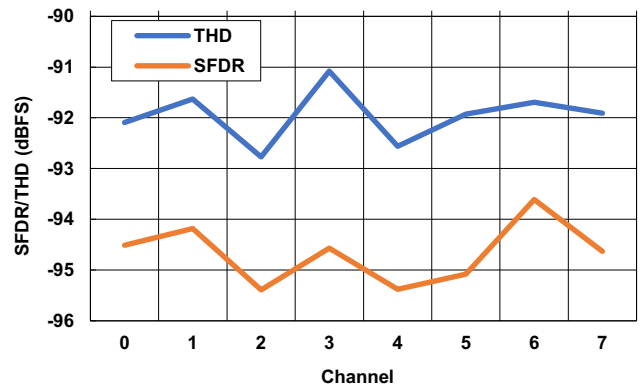
Figure 72. SFDR and THD vs Channel
