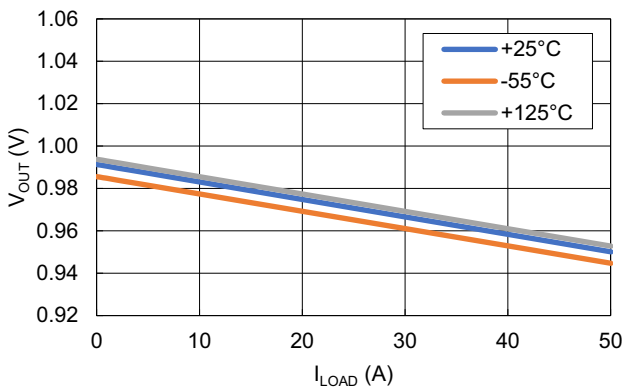
Figure 10. Droop Regulation for Various Temperatures ( V_{\text{IN}} = 5\text{V}, R_{\text{DROOP}} = 604\Omega )
