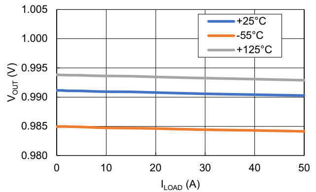
Figure 9. Load Regulation for Various Temperatures ( V_{\text{IN}} = 12\text{V} )
