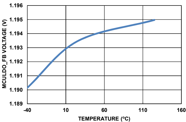
FIGURE 111. V_{MCULDO\_FB}
