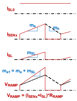
FIGURE 136. SLOPE COMPENSATION BLOCK DIAGRAM
