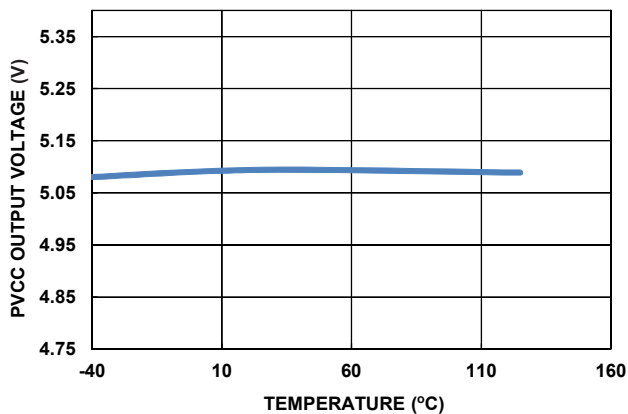
FIGURE 117. PVCC OUTPUT VOLTAGE vs TEMPERATURE
