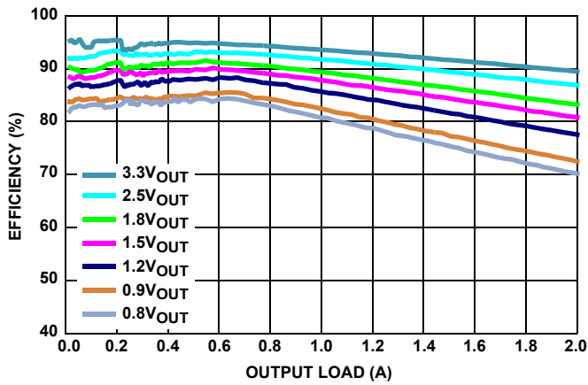
図 10. 効率 vs 負荷 F_{SW} = 1\text{MHz} , V_{IN} = 5\text{V} , \text{MODE} = \text{PFM} , T_A = +25^\circ\text{C}
