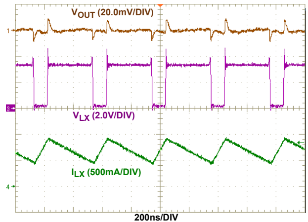
FIGURE 9. SWITCHING WAVEFORM PWM MODE, V_{IN} = 2.7V , I_{OUT} = 500mA , V_{OUT} = 3.3V
