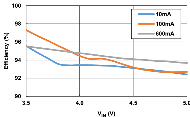
Figure 9. Efficiency vs Input Voltage: V_{OUT} = 3.3V
