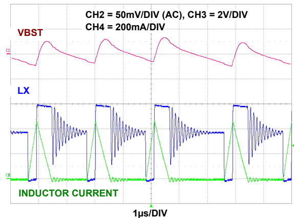
FIGURE 17. VBST RIPPLE, 50mA LOAD, VBST = 5.65V
