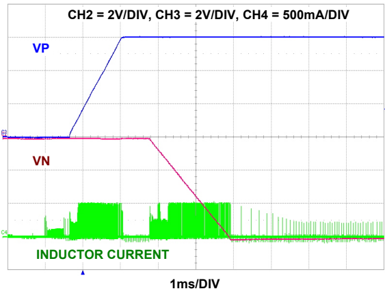
FIGURE 54. VP AND VN ( \pm 6\text{V} ) SOFT-START AT 3.7V INPUT VOLTAGE, VP/VN SEQUENCED (Reg 0x04 <math>b_4</math> = 0)
