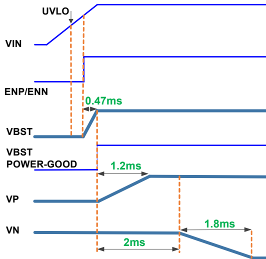
FIGURE 82. POWER-ON SEQUENCE - ACTIVATED BY ONE GPIO FOR ENN AND ENP, REGISTER 0x04 <b 4 > = 0 AND 0x05 <b 7 > = 0
