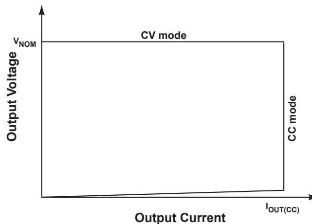
Figure 10.4 : Power Envelope
