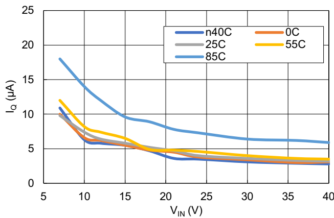
Figure 27. I_Q vs V_{IN} (In Regulation, No Load): RAA211403
