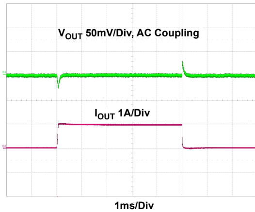
Figure 42. Load Transient I_{OUT} = 0A \rightarrow 1A \rightarrow 0 , Slew Rate 0.5A/\mu s
